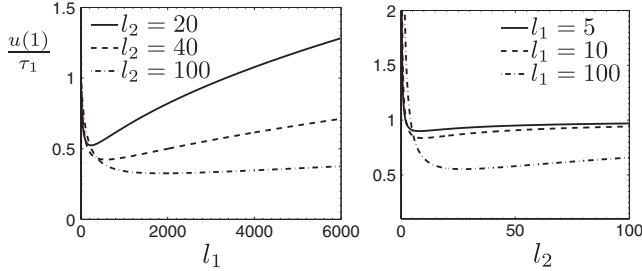
FIG. 3. Graph of the exit time u(1) from Eq. (9) as a function of l_1 and l_2 for \kappa = 0.1 , scaled by \tau_1 .
