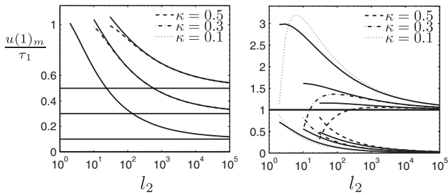
FIG. 4. The left panel displays the minimum u(1)_m scaled by \tau_1 as a function of l_2 and \kappa . The horizontal lines are \kappa , and the continuous curves are calculated using Eq. (10). The graphs do not extend up to l_2 = 0 because a minimum exists only for l_2 > \tilde{l}_2(\kappa) (see text). The right panel shows the ratio u_1(1)_m/\tau_1 (curves below the horizontal line) and u_2(1)_m/\tau_2 (curves above) of the corresponding sojourn times. The continuous curves are calculated using Eq. (10).
