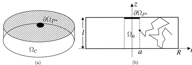
FIG. 2. (a) Elementary cylindrical compartment with a P^* molecule located centrally on the upper surface. (b) Cross-sectional view of the compartment. A cGMP molecule is hydrolyzed when reaching the boundary of the volume \Omega_a at r=a .
