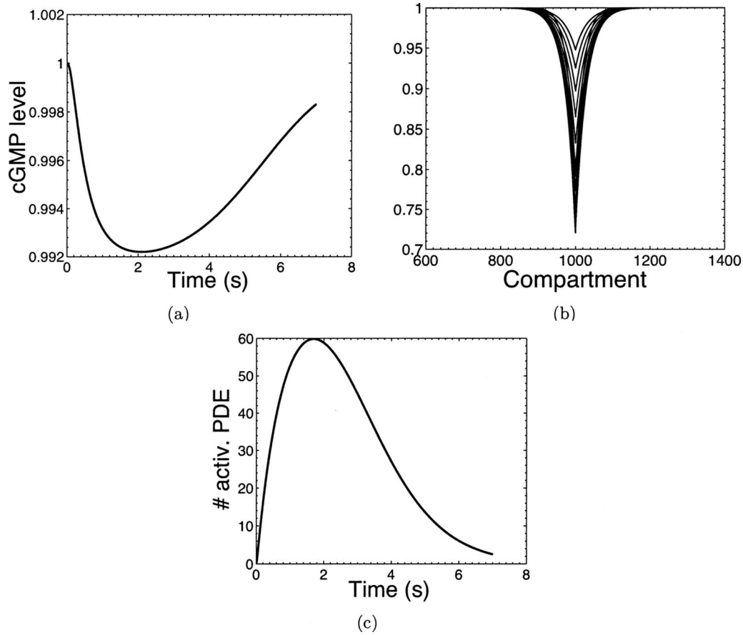
FIG. 3. cGMP dynamics after a photon absorption at time t=0 in compartment n=1000 ( N_c=2000 ). The simulation is performed using Eqs. (35) and (36). The cGMP concentration is scaled with the equilibrium value. (a) Time dependent cGMP level averaged over the outer segment. (b) cGMP level per compartment for various time points. (c) Number of light-activated PDE molecules obtained using the equations published in Ref. 34.
