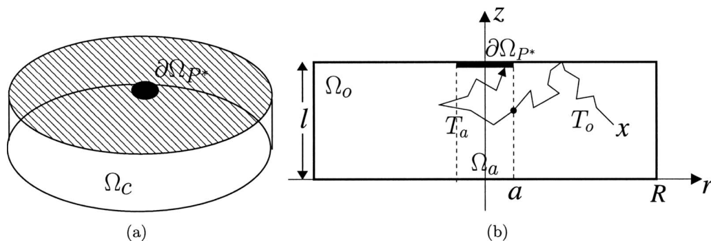
FIG. 4. (a) Cylindrical compartment \Omega_c with an activated PDE molecule located centrally on the upper surface. (b) The first time a cGMP molecule hits \partial\Omega_{P*} , when starting at position x in \Omega_o , is given by the sum of two times. First, the time T_o for a molecule starting at x to arrive at the boundary \partial\Omega_a , and second, the time T_a for the particle starting at \partial\Omega_a to arrive at \partial\Omega_{P*} .
