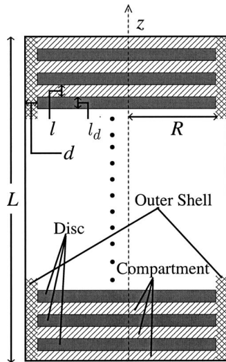
FIG. 1. Section through a cylindrical rod outer segment, containing a densely packed stack of parallel and uniformly distributed disks. The volume delimited by two adjacent disks is called a compartment.
