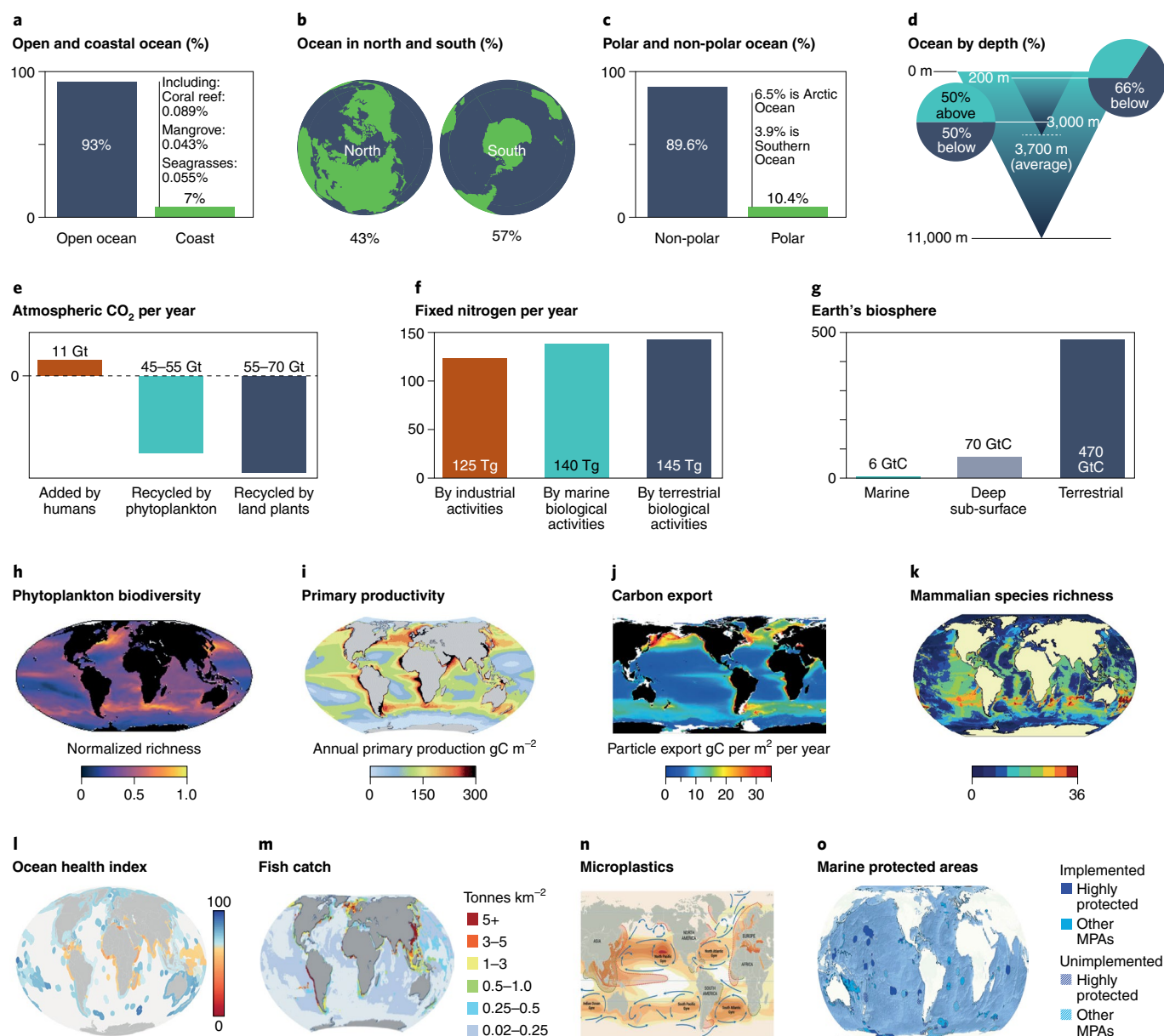
Fig. 4 | Key features related to the ocean microbiome. a–g. The extent of open ocean ( a ), particularly in the Southern Hemisphere ( b ) and in polar regions ( c ), is particularly understudied, as is the deep ocean ( d ), even though they represent huge extents of the ocean. In terms of global biogeochemical cycling, the ocean microbiome participates in almost as much recycling of atmospheric CO 2 by photosynthesis as all land plants combined ( e ). The ocean microbiome also fixes as much nitrogen as terrestrial ecosystems ( f ), despite contributing a much smaller biomass to the Earth's biosphere ( g ). For comparison, human contributions to atmospheric CO 2 and fixed nitrogen are indicated in e and f . h–o , Global maps show phytoplankton biodiversity (eukaryotic and prokaryotic groups combined; data from ref. 69 ) ( h ), primary productivity (data from https://www.grida.no/resources ) ( i ), carbon export (data from ref. 70 ) ( j ), marine mammal species richness (ref. 71 ) ( k ), ocean health index (data from http://www.oceanhealthindex.org/ ) ( l ), fish catch (data from 2004 at https://www.grida.no/resources ) ( m ), microplastics distribution (data from https://www.grida.no/resources ) ( n ) and coverage of marine protected areas (MPAs) (data from https://www.grida.no/resources ) ( o ). Other data sources: a , percent of open ocean versus coastal waters ( https://www.grida.no/resources ) (for seagrasses, mangroves and coral reefs 72–74 ); b , percent of ocean in Northern and Southern hemispheres 75 ; c , percent of polar ocean 76 ; d , percent of ocean at different depths 77 ; e, f , carbon and nitrogen fixation 2,78,79 ; and g , Earth's biosphere 180 . Panels a–c , l and n consider only surface area. Figure reproduced with permission from: b , ref. 75 , under a Creative Commons license CC BY 4.0; h , ref. 69 , under a Creative Commons license CC BY 4.0; i, m , Hugh Ahlenius, UNEP/GRID-Arendal; j , ref. 70 , Wiley; k , Nordpil.com; l , ref. 81 , Springer Nature Ltd; n , Riccardo Pravettoni and Philippe Rekacewicz/GRID-Arendal; o , Kristina Thygesen/GRID-Arendal.
